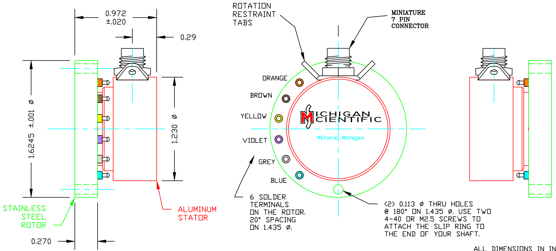
FRONT VIEW OF MATING CONNECTOR & COLOR OF ROTOR TERMINAL
