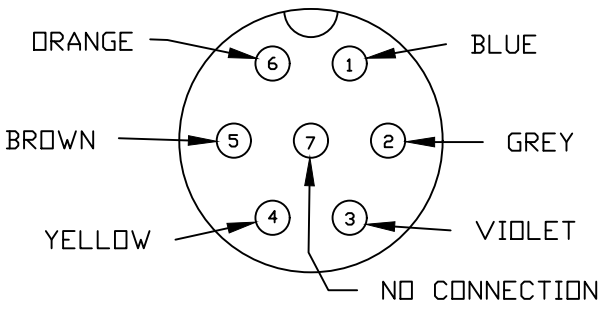
FRONT VIEW OF MATING CONNECTOR & COLOR OF ROTOR TERMINAL
